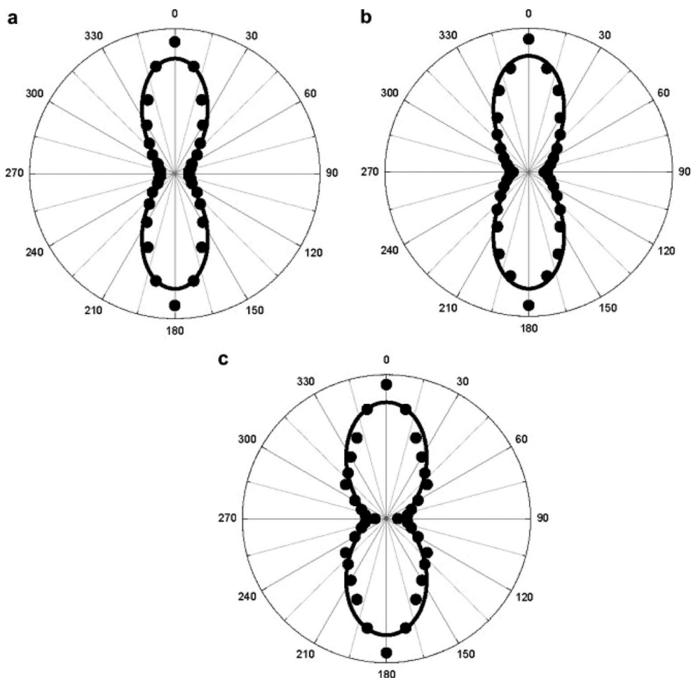
Figure 16. Polar plots of the HRS intensities as a function of the incident light (1907 nm) polarization angle \Psi for the copper nanoparticles of diameters (a) 25 nm, (b) 55 nm, and (c) 100 nm. Solid circles are the HRS intensities, and solid lines are fits to the data points. Reprinted with permission from ref 70. Copyright 2009 Elsevier.
