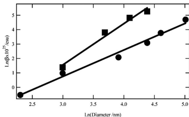
Figure 6. Log–log plot of the hyperpolarizability magnitude against the particle diameter for silver (■) and gold (●) particles at the harmonic wavelengths of 390 and 400 nm, respectively. Reprinted with permission from ref 55. Copyright 2007 American Chemical Society.
