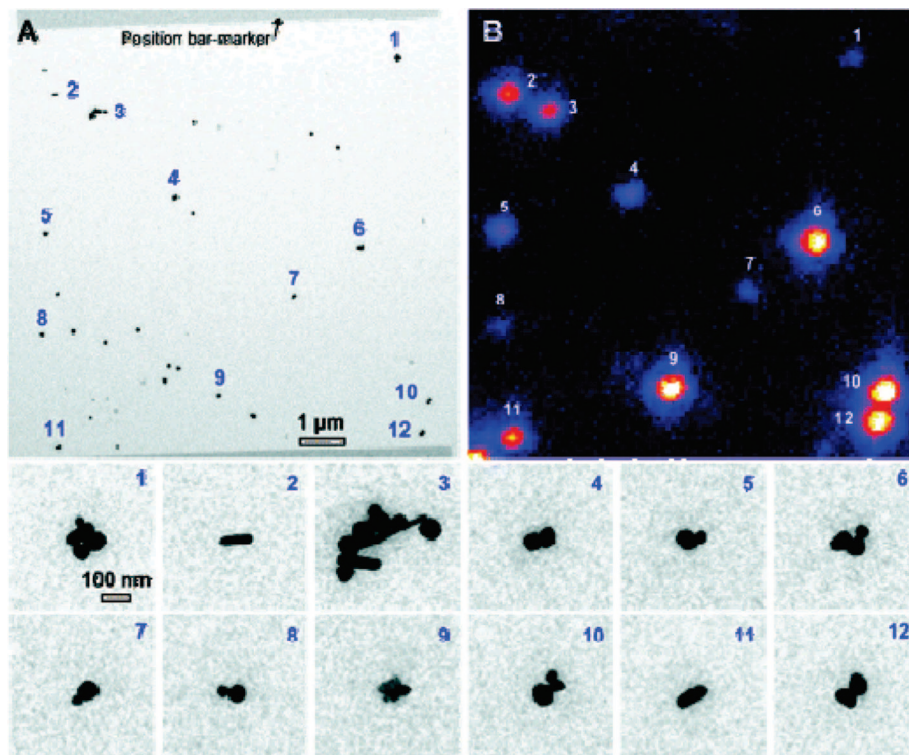
Figure 24. (A) TEM image of Ag nanoparticles. (B) SHG map (false color image, with white showing the most intense 415-nm signal) of the same area ( \lambda_{\text{ex}} = 830 nm, 3 mW average power, 40 GW/cm 2 peak power). The bottom panel shows the zoomed-in images of the labeled particles. Reprinted with permission from ref 87. Copyright 2005 American Chemical Society.
