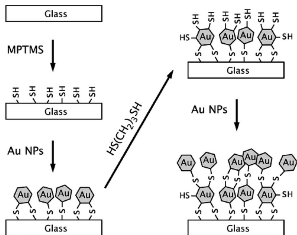
Figure 29. Schematic showing the construction of the nanoparticle substrates using the alternate immersion of solutions of gold nanoparticles and a dithiol linker molecule. Reprinted with permission from ref 159. Copyright 2009 American Chemical Society.
