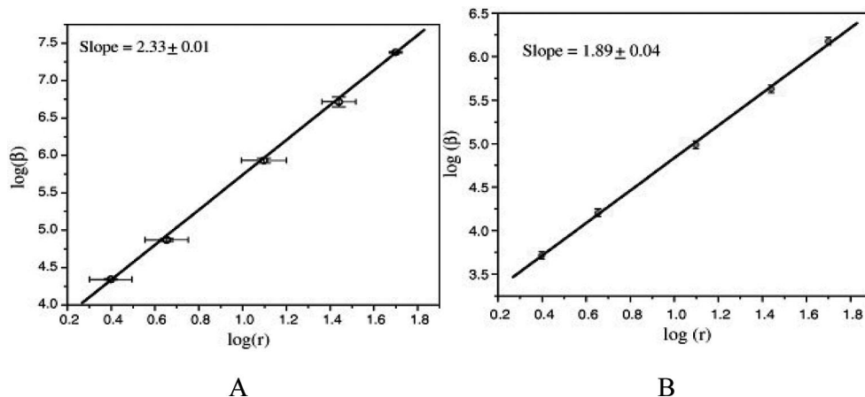
Figure 13. (A) log–log plot of \beta /particle (at 1064 nm excitation wavelength) vs particle size, r , for copper nanoparticles. The straight line is a linear fit to the data points. (B) Size dependence of the first hyperpolarizability of copper nanoparticles at 1907 nm. Reprinted with permission from ref 69. Copyright 2009 Elsevier.
