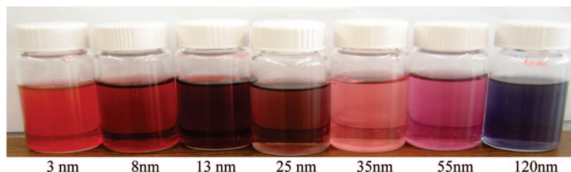
Figure 1. Photograph showing gold nanoparticles of different sizes. Reprinted with permission from ref 75. Copyright 2009 Wiley-VCH.
