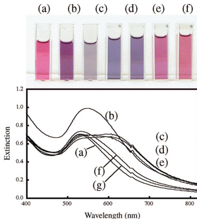
Figure 50. Colorimetric responses (top panel) and corresponding spectral traces (bottom panel) from (a) Au-MUA, (b) Au-MUA/ Pb^{2+} , and (c–g) Au-MUA/ Pb^{2+} and increasing amounts of EDTA. The Pb^{2+} concentration in sample b is 0.67 mM; the EDTA concentrations in samples c–g are 0.191, 0.284, 0.376, 0.467, and 0.556 mM. Reprinted with permission from ref 46. Copyright 2001 American Chemical Society.
