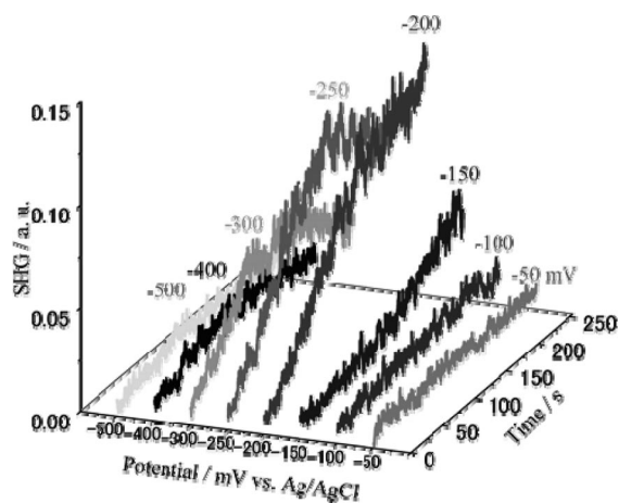
Figure 40. Three-dimensional plot of time-dependent p-in/p-out SHG intensity transients at the p-GaAs(001) electrode in a 0.1 M \text{H}_2\text{SO}_4 solution containing 1 mM of \text{CuSO}_4 . The azimuthal angle was fixed at 90^\circ . The electrode potential was stepped from +100 mV to each deposition potential at t = 0 s. Reprinted with permission from ref 173. Copyright 2005 American Chemical Society.
