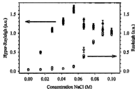
Figure 27. Effect of NaCl addition upon Rayleigh and hyper-Rayleigh scattering signal intensities. The scattering scales are arbitrary. Reprinted with permission from ref 43. Copyright 1998 American Chemical Society.
