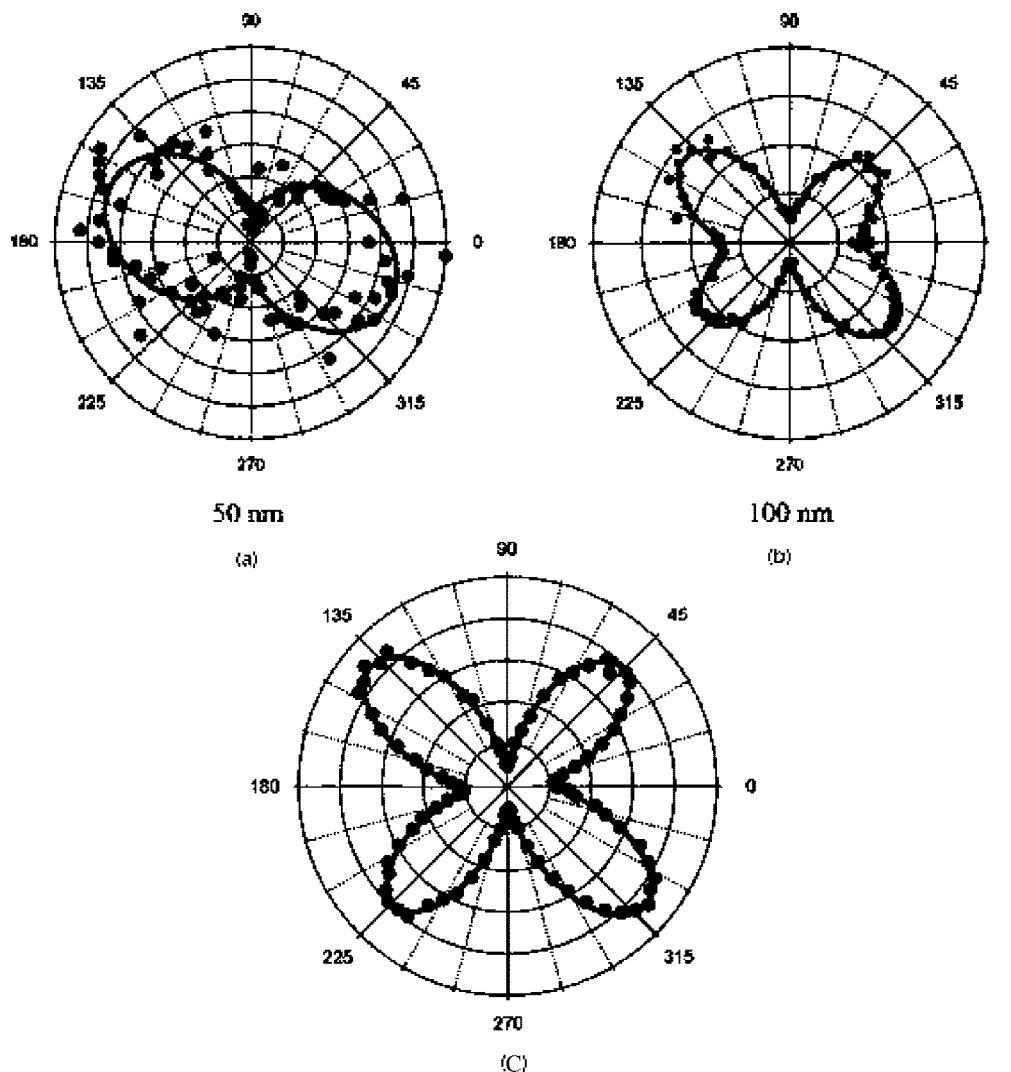
Figure 8. Polar plot of the HRS intensity as a function of the incoming fundamental beam polarization angle: (filled circles) experimental points and (solid) fit to the experimental data points using theoretical modeling for an aqueous suspension of (a) 50 nm diameter, (b) 100 nm diameter, and (c) 150 nm diameter gold particles. Reprinted with permission from ref 57. Copyright 2006 American Institute of Physics.
