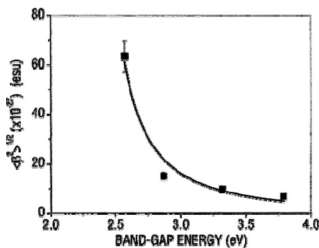
Figure 18. First hyperpolarizability \langle\beta^2\rangle^{1/2} as a function of the band gap energy for the investigated samples of colloidal suspensions of \text{Cd}_x\text{Zn}_{1-x}\text{S} nanocrystals. The points are experimental data, whereas the solid line is the best-fitting curve. Reprinted with permission from ref 170. Copyright 2002 American Chemical Society.
