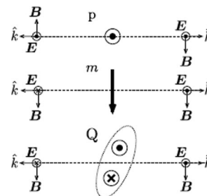
Figure 10. Simple schematic of the radiative properties of an electric dipole ( p ), a magnetic dipole ( m ), and a quadrupole ( Q ). Reprinted with permission from ref 50. Copyright 2007 American Physical Society.
