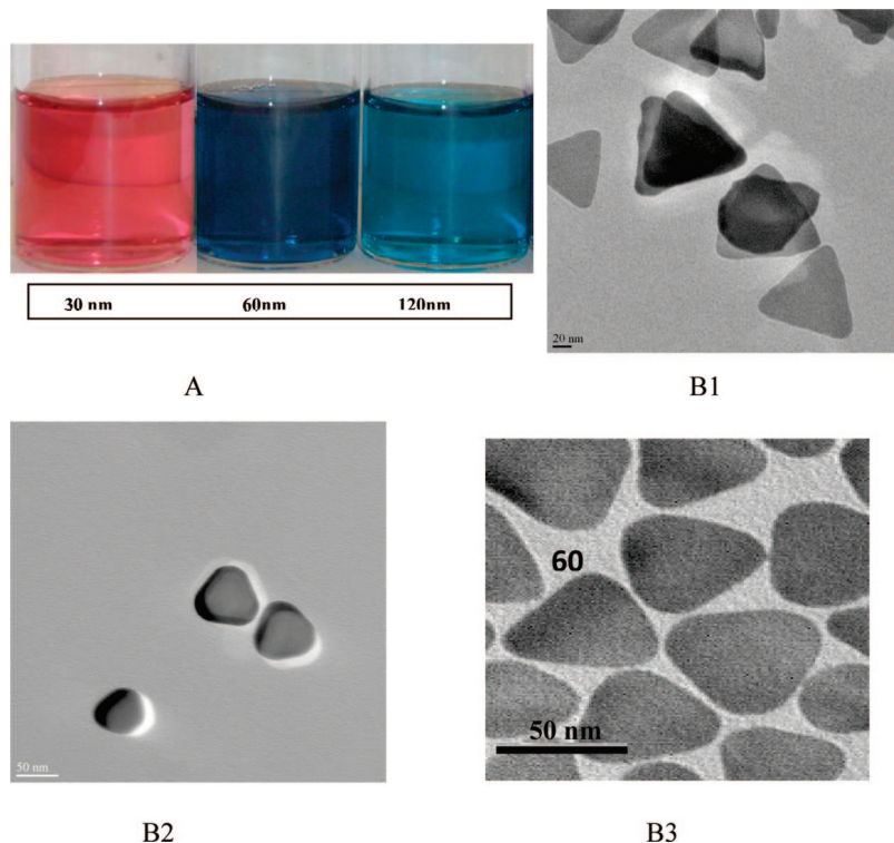
Figure 3. (A) Photographic images. (B1–B3) TEM pictures of silver nanoprisms of different sizes (30 nm, 60 and 120 nm edge length). Reprinted with permission from ref 157. Copyright 2009 Elsevier.
