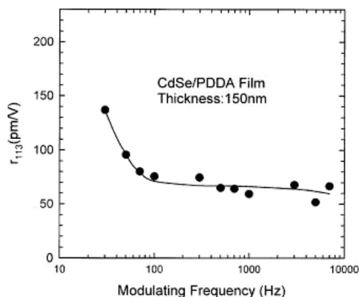
Figure 19. r_{113} as a function of modulating frequency measured using the Mach–Zehnder setup. Symbols and solid line indicate the measured and fitted results, respectively. Reprinted with permission from ref 96. Copyright 2002 American Institute of Physics.
