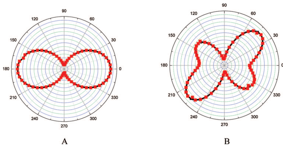
Figure 12. (A) Polar plot of the HRS intensity as a function of the incoming fundamental beam polarization angle ( \varphi ) from aqueous suspensions of 30 nm silver nanoparticles. Solid points are the HRS experimental data, and solid lines are the theoretical fit of the experimental data point using eq 18. (B) Polar plot of the HRS intensity as a function of the incoming fundamental beam polarization angle from aqueous suspensions of 80 nm silver nanoprisms. Solid points are the HRS experimental data, and solid lines are the theoretical fit of the experimental data point using eq 19. Reprinted with permission from ref 157. Copyright 2009 Elsevier.
