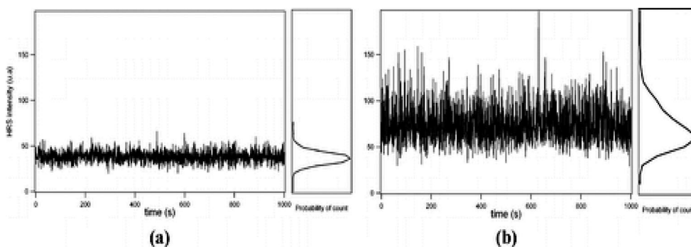
Figure 23. (a) (left) HRS counts for 0.5 s periods as a function of time recorded for a bare water cell. (right) Histogram of the counts. (b) (left) HRS counts for 0.5 s periods as a function of time recorded for a 31 fM concentration of 80 nm diameter silver nanoparticles. (right) Histogram of the photon counts. Reprinted with permission from ref 62. Copyright 2009 American Chemical Society.
