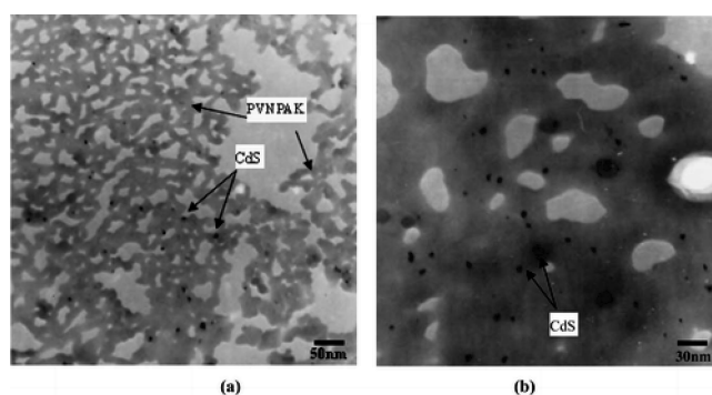
Figure 37. TEM images of PVNPAK-5-CdS (a) and PVNPAK-15-CdS (b) nanocomposites. The chemically hybridized CdS-PVNPAK nanocomposite samples were prepared by the sulfonation of PVNPAK, the preparation of the precursor PVNPAK(SO 3 ) 2 Cd, and the in situ formation of CdS-PVNPAK nanocomposites. Reprinted with permission from ref 161. Copyright 2008 American Chemical Society.
