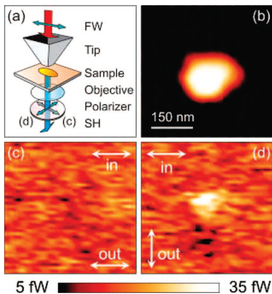
Figure 26. Polarization of the SH generated by nanoparticles with a 150 nm major axis: (a) experimental geometry (the FW light is polarized parallel to the particle major axis); (b) topography; (c) and (d) SH emission map with a polarizer on detection parallel (c) and perpendicular (d) to the particle major axis. Image size: 0.45 \times 0.45 \mu\text{m}^2 . Reprinted with permission from ref 158. Copyright 2008 American Institute of Physics.
