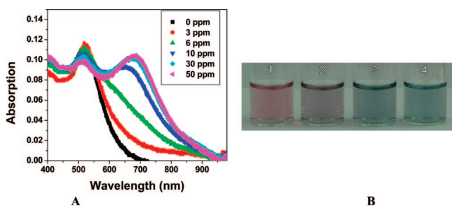
Figure 52. (A) Absorption profile of modified gold nanoparticles before and after the addition of different concentrations of \text{Hg}(\text{II}) ions. (B) Photographic images of the color of MPA-PDCA modified gold nanoparticles (13 nm) in the presence of different concentrations of \text{Hg}(\text{II}) ion: (1) 3 ppm, (2) 6 ppm, (3) 10 ppm, (4) 50 ppm. Reprinted with permission from ref 71. Copyright 2008 American Chemical Society.
