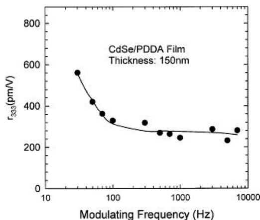
Figure 20. r_{333} as a function of modulating frequency measured using the Mach–Zehnder setup. Symbols and solid line indicate the measured and fitted results, respectively. Reprinted with permission from ref 96. Copyright 2002 American Institute of Physics.
