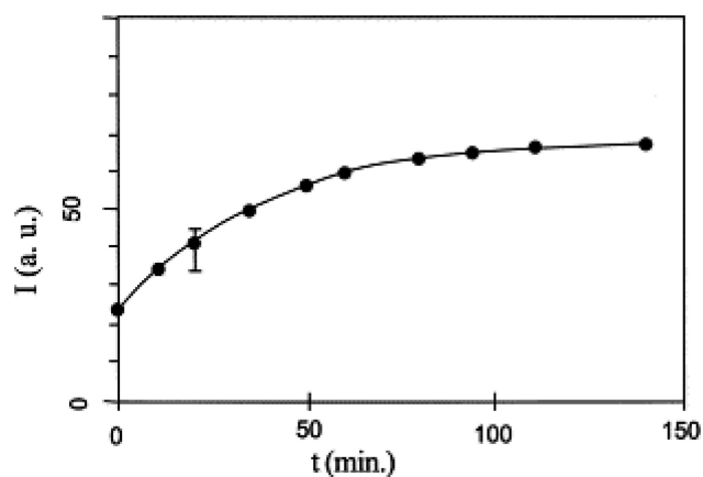
Figure 39. Kinetics of formation of \text{TiO}_2 nanoparticles as monitored by HRS of 800 nm radiation. Reprinted with permission from ref 73. Copyright 2002 Elsevier.
