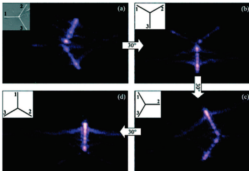
Figure 22. SH images of the tetrapod with different orientations relative to the polarization of the fundamental excitation. The polarization of the fundamental wave is kept vertical. The tetrapod is rotated 30^\circ clockwise per step from (a) to (d). The orientation of leg 1 starts to be perpendicular to the fundamental wave's polarization and ends parallel to that. Reprinted with permission from ref 172. Copyright 2009 American Chemical Society.
