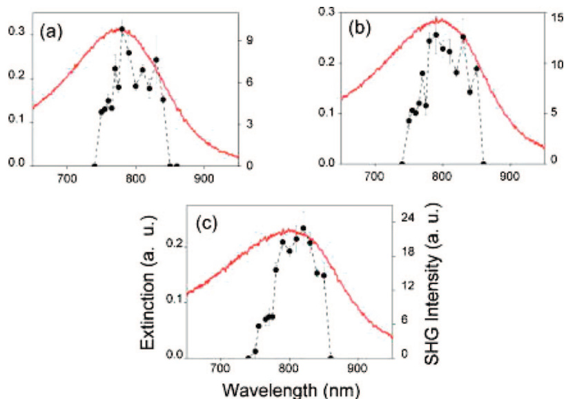
Figure 11. Second-harmonic generation enhancement (circles) from arrays of gold nanorods with a (a) 150 nm, (b) 170 nm, and (c) 190 nm long axis (the dashed line serves as a guide for the eyes). The extinction spectrum (solid line) is shown for comparison. The irradiation time and power used to record the second harmonic signal were equal to 5 s and 50 mW, respectively. The incident polarization was set parallel to the nanoparticle long axis. Reprinted with permission from ref 156. Copyright 2007 American Institute of Physics.
