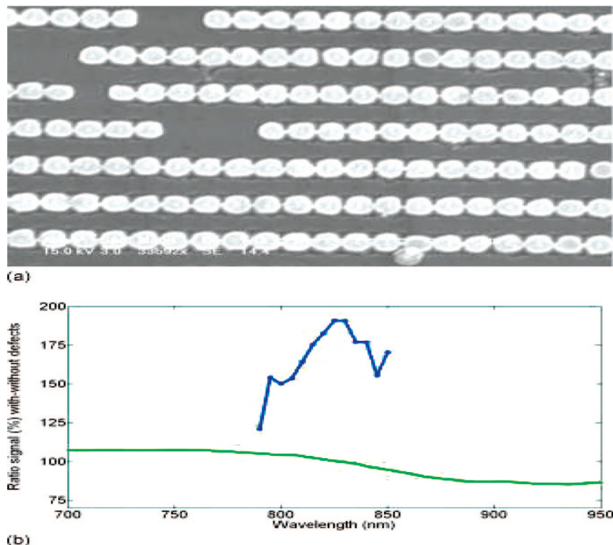
Figure 31. (a) SEM image of the array with 10% random defects. (b) Ratio of the SHG and linear optical reflectivity between the arrays without and with defects. Reprinted with permission from ref 160. Copyright 2008 American Institute of Physics.
