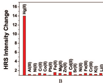
Figure 54. (A) Photographic images of the color of MPA-HCys-PDCA modified gold nanoparticles in the presence of different metal ions of 40 ppm concentration. (B) HRS intensity change upon the addition of 40 ppm of different metal ions to a gold nanoparticle-MPA-HCys-PDCA solution (5 nM). Reprinted with permission from ref 71. Copyright 2008 American Chemical Society.
