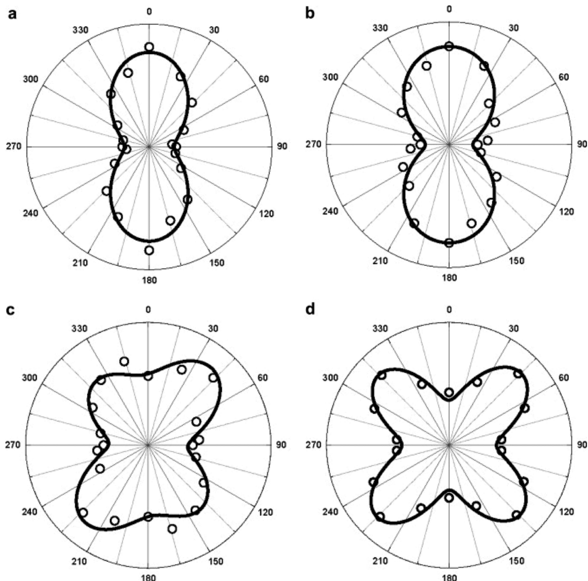
Figure 15. Polar plots of the HRS intensities as a function of the incident light (738 nm) polarization angle \Psi for the Cu nanoparticles of diameters (a) 9 nm, (b) 25 nm, (c) 55 nm, and (d) 100 nm. Open circles are the HRS intensities, and solid lines are fits to the data points. Reprinted with permission from ref 70. Copyright 2009 Elsevier.
