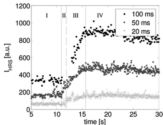
Figure 38. HRS signals during the early stages of precipitation monitored for three different time resolutions (circles, 100 ms; squares, 50 ms; crosses, 20 ms). Four different regions can be discerned: (I) only one reactant; (II) nucleation; (III) growth; (IV) ripening. Note that the absence of data points (100 ms resolution) between 11 and 13 s was due to drop-out of the laser. Reprinted with permission from ref 58. Copyright 2009 American Chemical Society.
