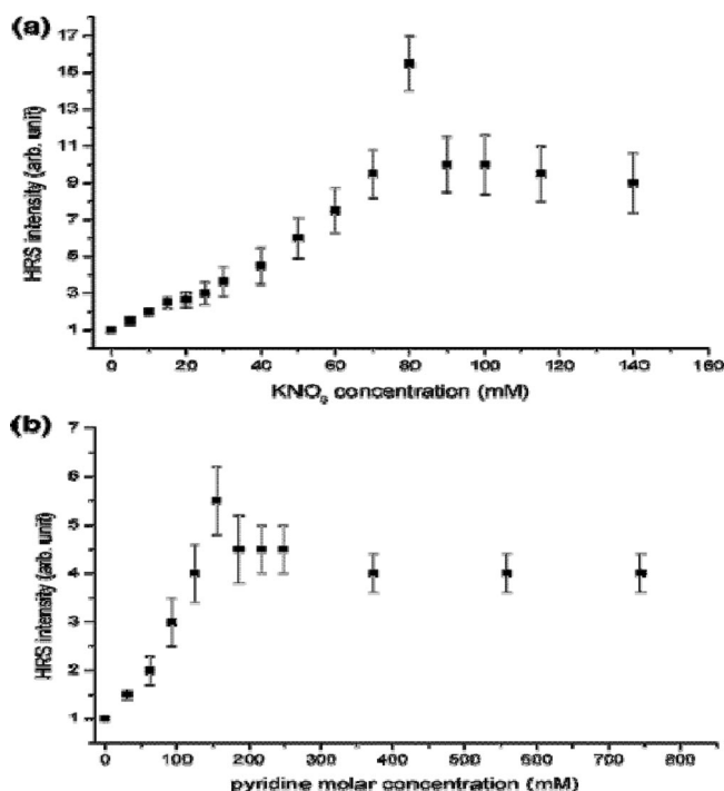
Figure 28. (a) HRS intensity as a function of \text{KNO}_3 concentration. (b) HRS intensity as a function of pyridine concentration. Reprinted with permission from ref 72. Copyright 2005 American Chemical Society.
