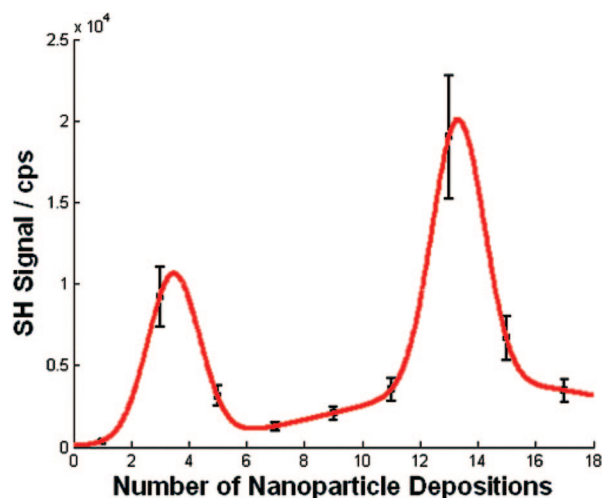
Figure 30. SHG signal of NP-containing substrates obtained using 820 nm fundamental radiation with a 200 fs pulse duration and a 10 nJ pulse energy at a 5 MHz repetition rate. Data was collected at a 45° incidence angle. p-Polarized radiation was used exclusively for the fundamental and the second harmonic. The maximum SHG signal is observed for 13 NP depositions. Reprinted with permission from ref 159. Copyright 2009 American Chemical Society.
