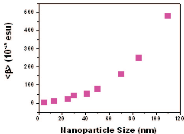
Figure 7. Variation of \langle\beta\rangle with particle size in water solvent. Reprinted with permission from ref 75. Copyright 2009 Wiley-VCH.
