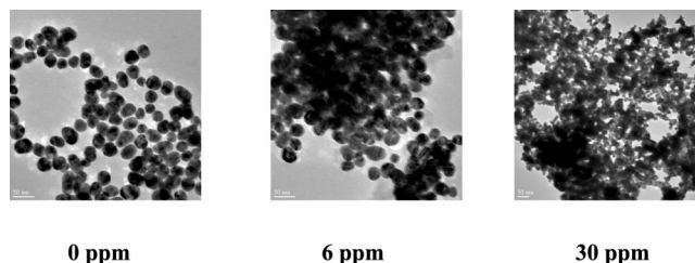
Figure 53. TEM images of MPA-PDCA modified gold nanoparticle solution in the presence and absence of \text{Hg}(\text{II}) ions. Reprinted with permission from ref 71. Copyright 2008 American Chemical Society.
