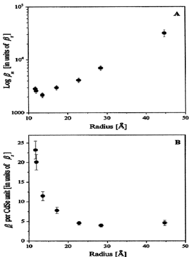
Figure 17. Size dependence of the SHG response from CdSe nanocrystals. Frame A shows, on a log scale, the size dependence of \beta_n , the value of the hyperpolarizability per nanocrystal, which decreases as size is decreased to radii of 13.5 Å. For the smallest radii, this trend is reversed and \beta_n increases. Frame B depicts the size dependence of the normalized value of the hyperpolarizability per unit cell, which shows significant systematic enhancement for small sizes. The primary contribution to the error bars is the uncertainty in the determination of nanocrystal concentrations from the measured extinction coefficients, as discussed in the Experimental Section. A \pm 20\% error in \epsilon propagates to \pm 10\% error in the values of \beta_n . Reprinted with permission from ref 76. Copyright 2000 American Chemical Society.
