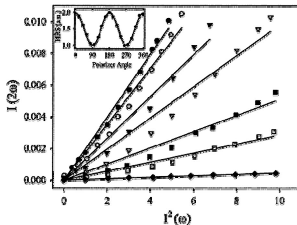
Figure 4. Power dependence of hyper-Rayleigh scattering, I(2\omega) , vs incident intensity squared, I^2(\omega) , for various concentrations of Au: (●) 2.1 \times 10^{17} \text{ cm}^{-3} ; (○) 8.4 \times 10^{16} \text{ cm}^{-3} ; (▼) 4.2 \times 10^{16} \text{ cm}^{-3} ; (▽) 2.1 \times 10^{16} \text{ cm}^{-3} ; (■) 8.4 \times 10^{15} \text{ cm}^{-3} ; (□) 4.2 \times 10^{15} \text{ cm}^{-3} ; (◆) water. Inset shows results of rotating a polarizer in front of the detector. Reprinted with permission from ref 43. Copyright 1998 American Chemical Society.
