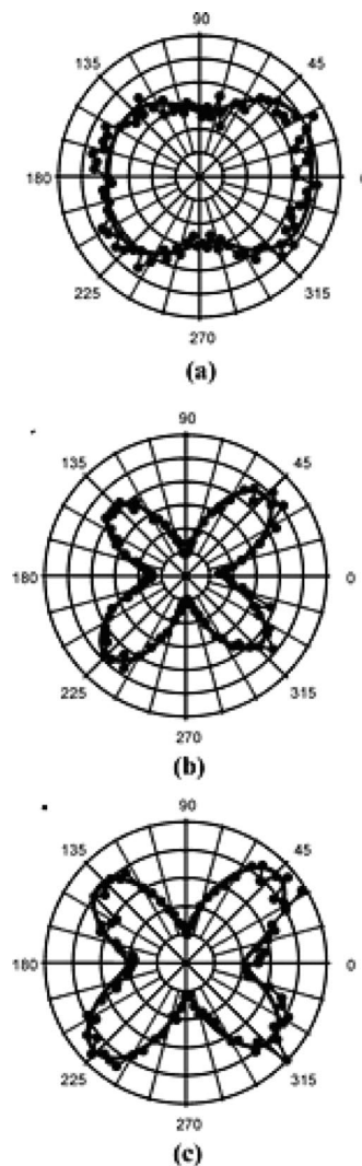
Figure 9. Polar plot of the HRS intensity as a function of the incoming fundamental beam polarization angle: (filled circles) experimental points and (solid) theoretical fit to the experimental data for aqueous suspensions of (a) 40 nm, (b) 60 nm, and (c) 80 nm diameter silver particles for a harmonic wavelength of 390 nm vertically polarized. Reprinted with permission from ref 55. Copyright 2007 American Chemical Society.
