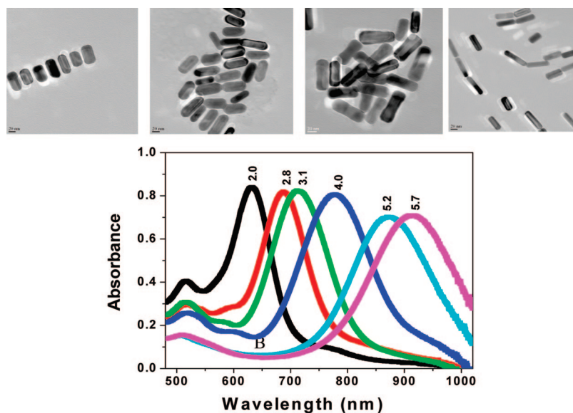
Figure 2. (A) TEM image of gold nanorods of average aspect ratios ( \sigma \approx 2.0, 2.8, 4.0, and 5.2 ). (B) Extinction profile of Au nanorods with aspect ratios varying from 2.0 to 5.7. The strong long wavelength band in the near-infrared region ( \lambda_{LPR} = 600\text{--}950 nm) is due to the longitudinal oscillation of the conduction band electrons. The short wavelength peak ( \lambda \approx 520 nm) is from the nanorods' transverse plasmon mode. Reprinted with permission from ref 81. Copyright 2008 Wiley VCH.
